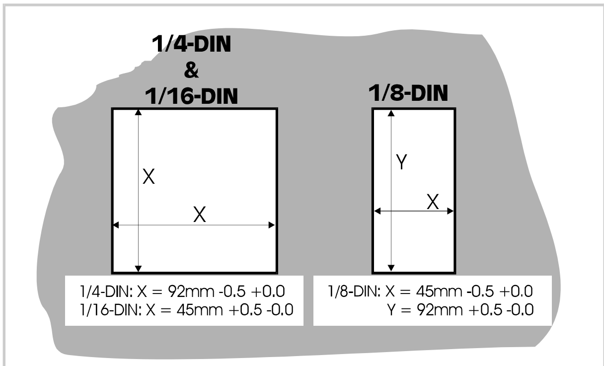
Figure 1-1 Cut-out Dimensions
