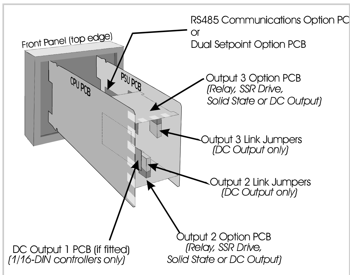
Figure 2-1 PCB Positions
