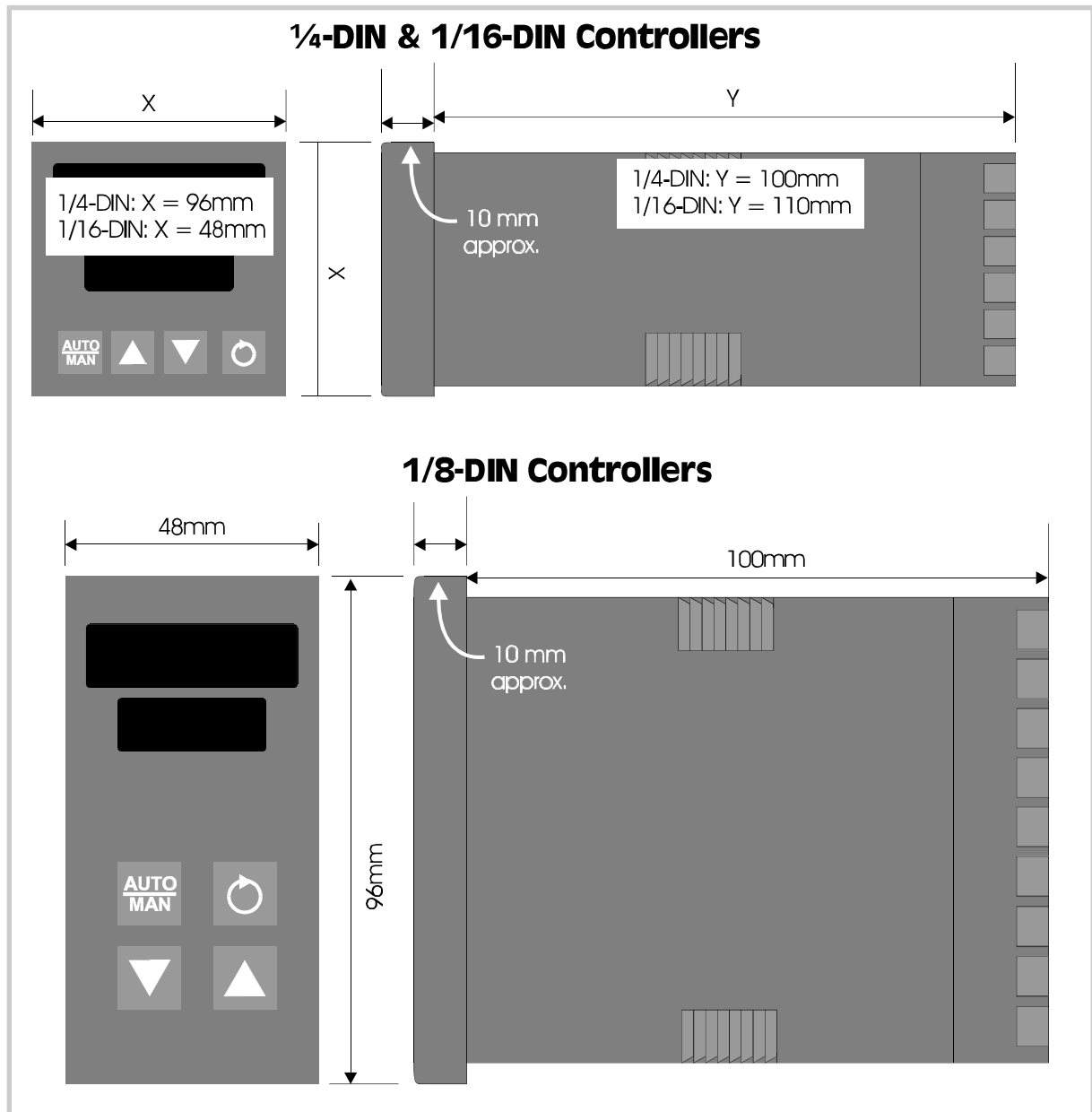
Figure 1-2 Main Dimensions
