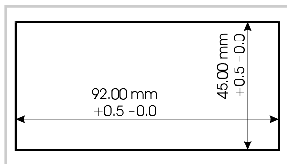
Figure 1-1 Panel Cut-out
