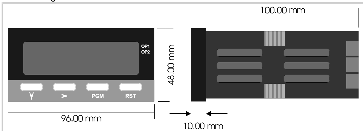
Figure 1-2 Main Dimensions
